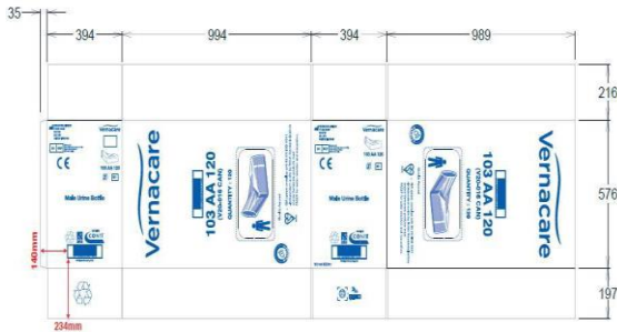
Outer Case Dimensions 576 x 994 x 394mm
